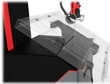
GROUND ARTICULATING TABLE MITERS 10° LEFT & 45° RIGHT FOR CONTOUR CUTTING
